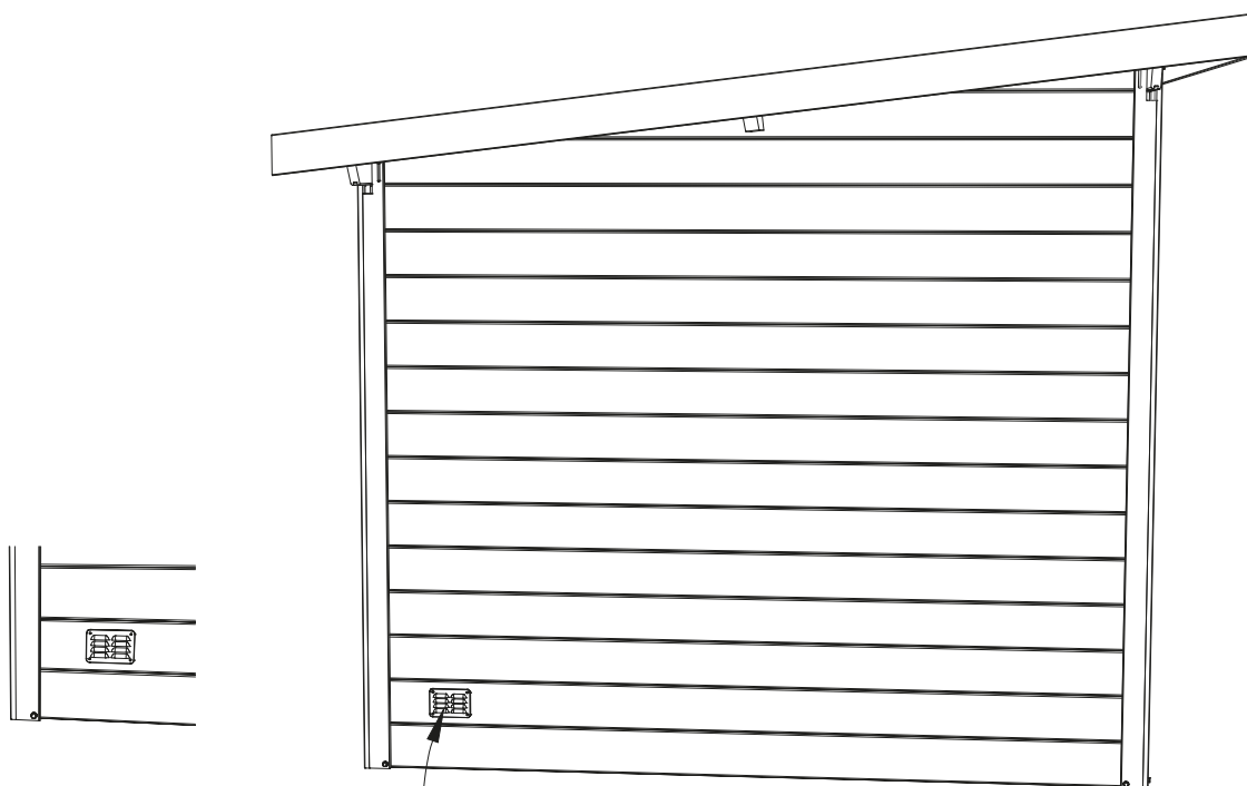
S6746 Ventilation-kit
